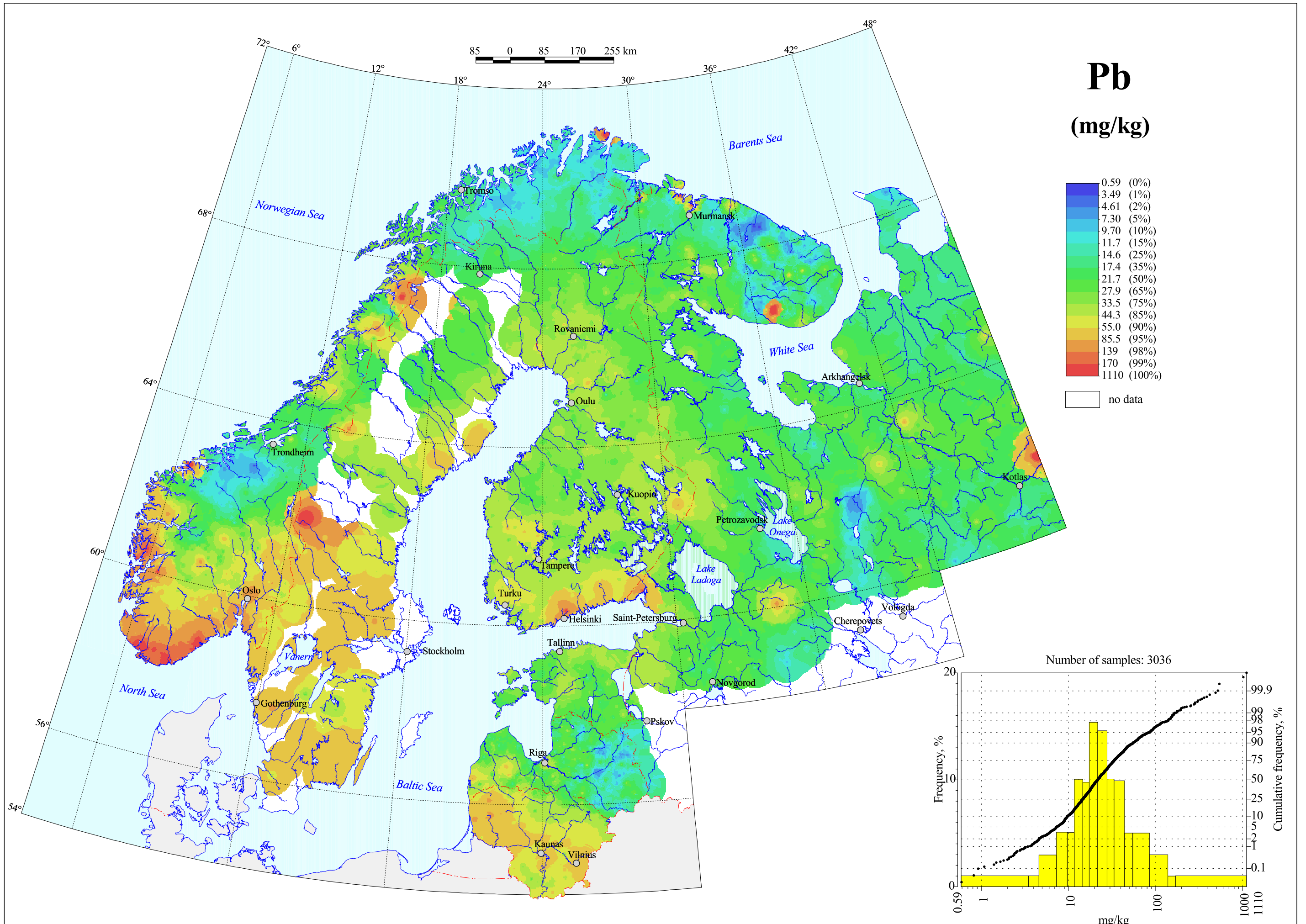
Lead in Organic Soil Layer, Total Content
